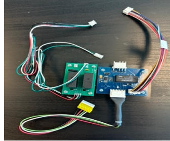
Billiards Adapter Board with C10 Harness
